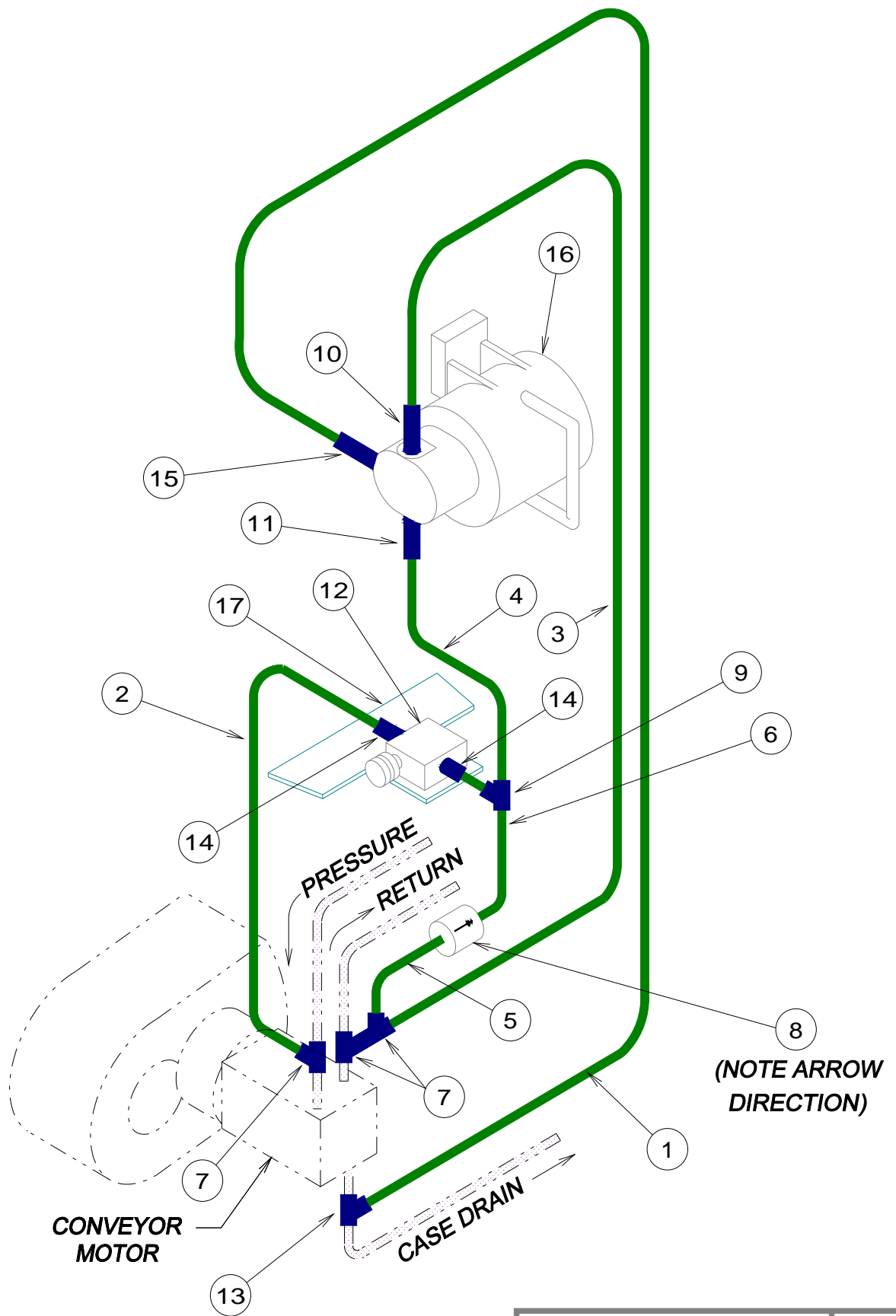
HYDRAULIC PLUMBING HOPPER VIBRATOR
